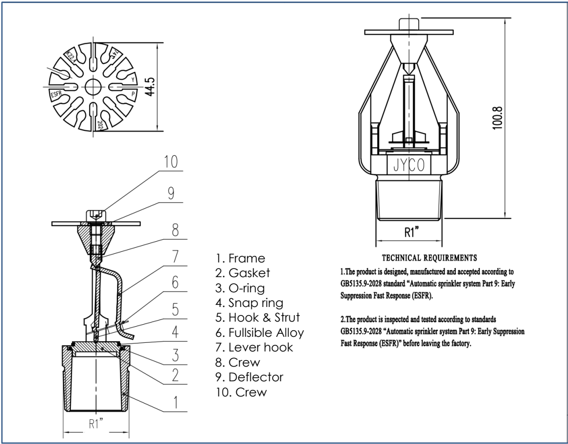
MODEL ESFR Pendent SPRINKLER, 22.4K EARLY SUPPRESSION, FAST RESPONSE
