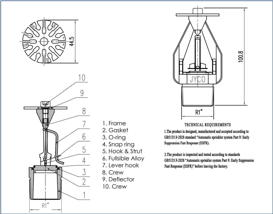
MODEL ESFR Pendent SPRINKLER, 25.2K EARLY SUPPRESSION, FAST RESPONSE
